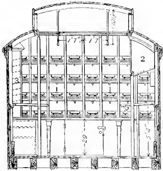
Fig. 609. Transverse Section.
